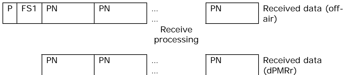
Figure 2 – dPMRr received data format
