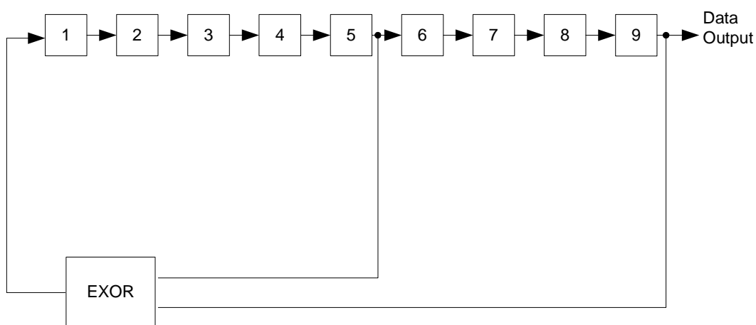
Figure 3 - 511 bit 9-bit PRBS generator
