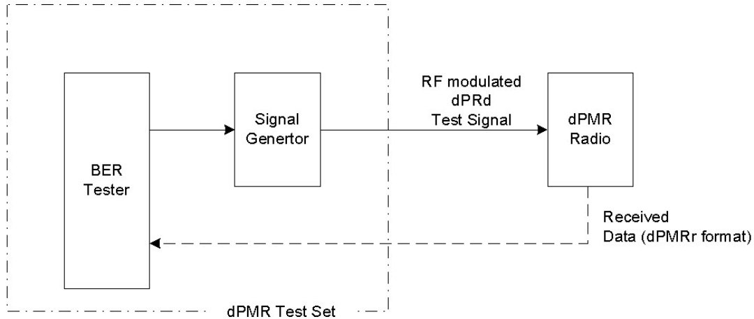
Figure 1 – Typical dPMR BER test configuration
